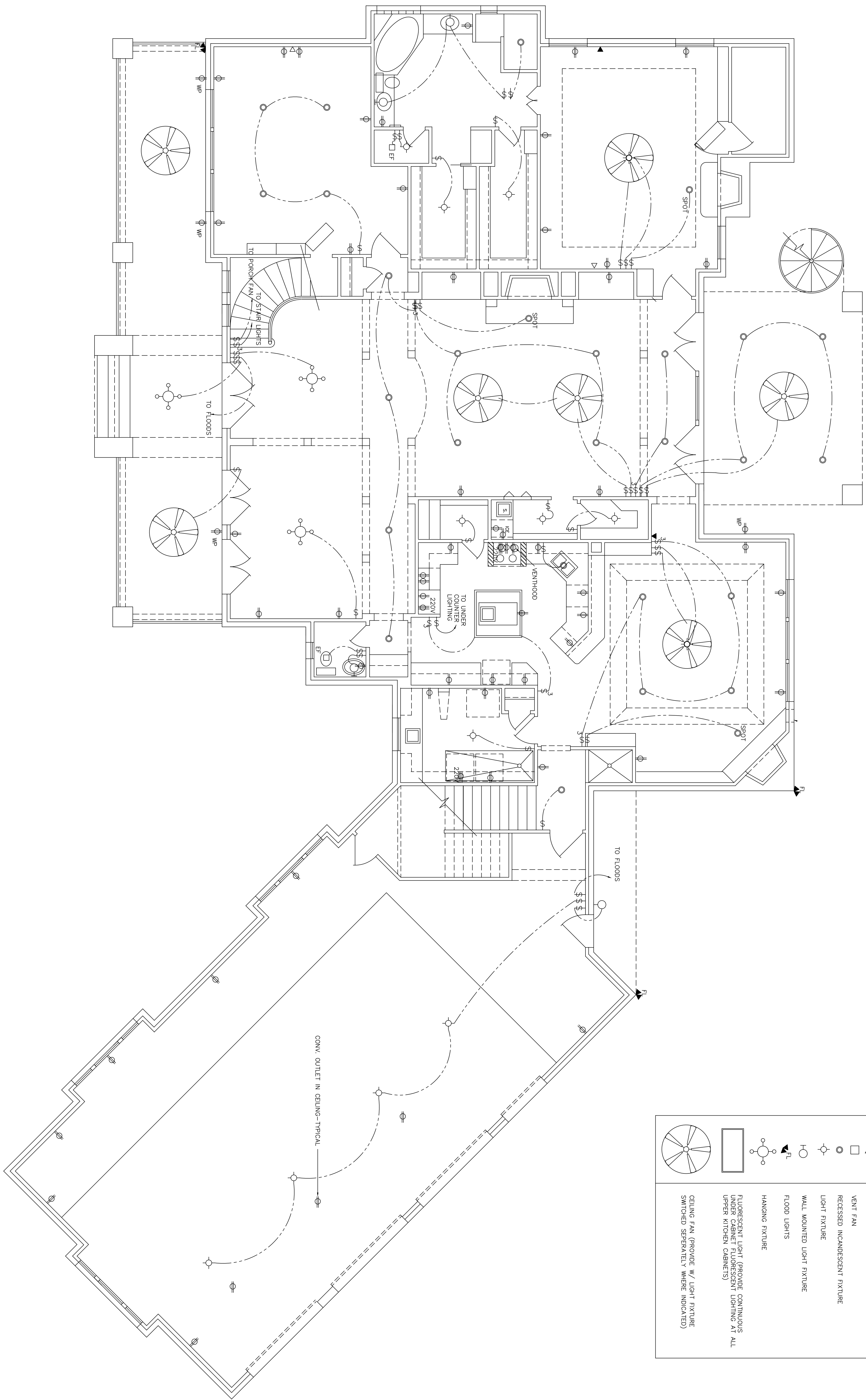
FIRST FLOOR ELECTRICAL PLAN SCALE: 1/4" = 1'-0"
